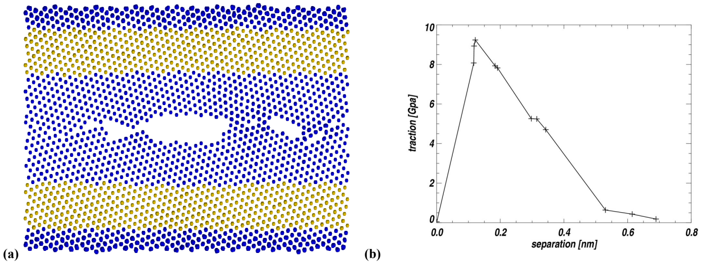
Figure 3. Decoherence of a [441] symmetric tilt grain boundary (i.e., the plane of the boundary is a [441] plane for each grain). (a) Snapshot from an MD simulation, highlighting those atoms used in the linear regression to determine the traction-separation relation. (b) Traction-separation curve derived from MD simulation.
